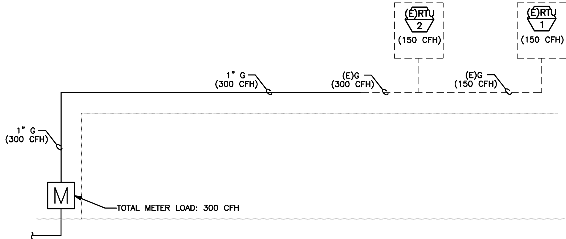
GAS PIPING RISER DIAGRAM
