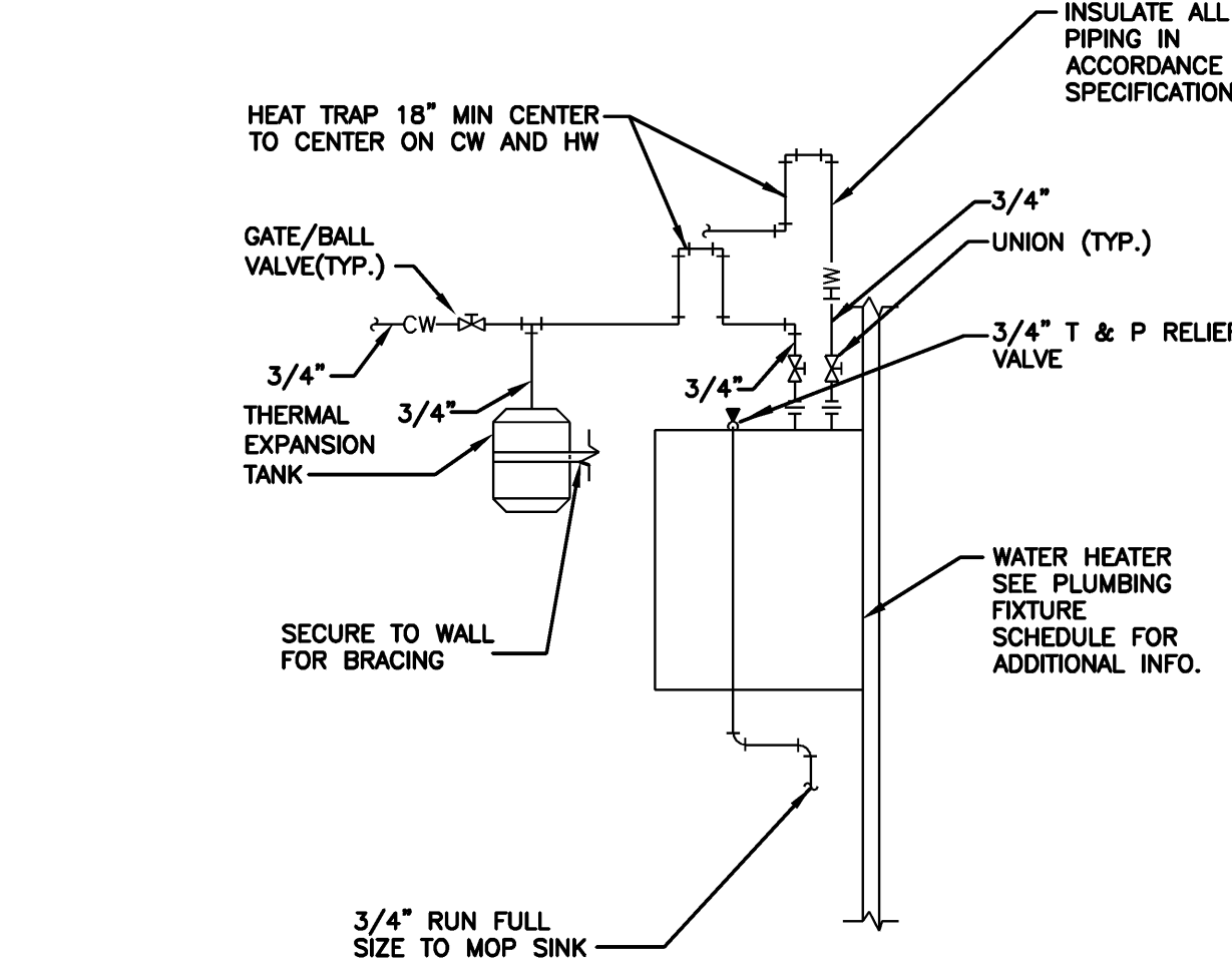
TANK WATER HEATER
